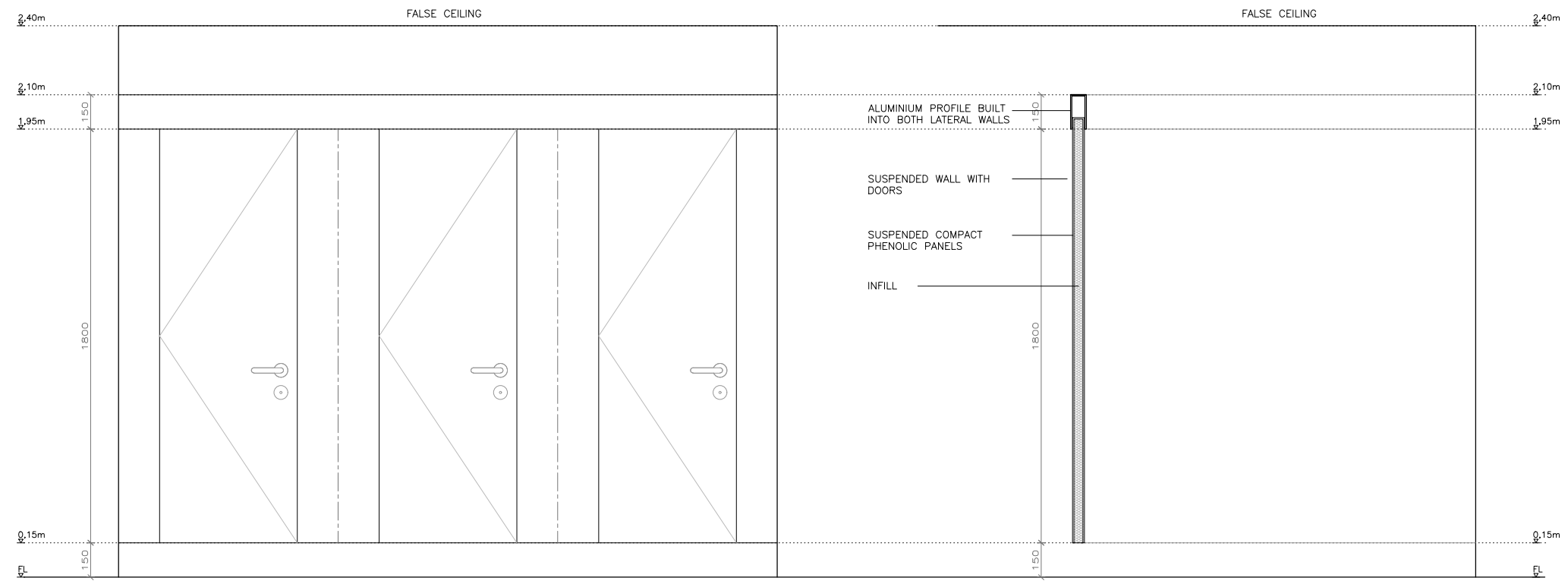
ELEVATION & SECTION OF TOILET CABINETS 1:25
